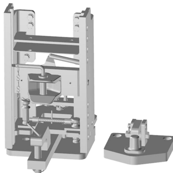
FP2500 SIR – semelles interchangeables
